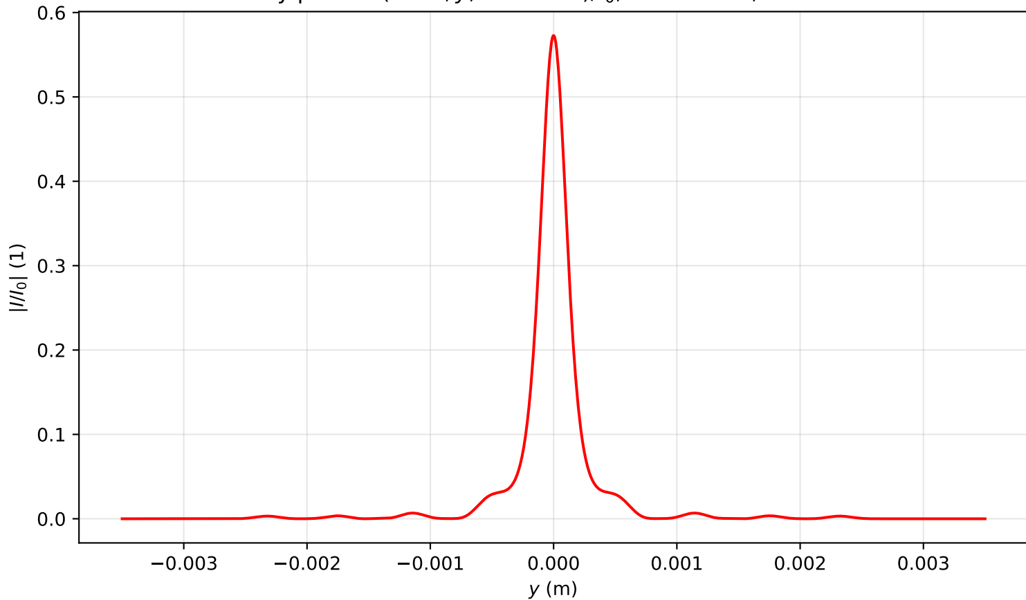
Intensity profile I(x=0, y, z=3.981)/I_0 , P_{in}=7.0P_{cr} , artificial time
